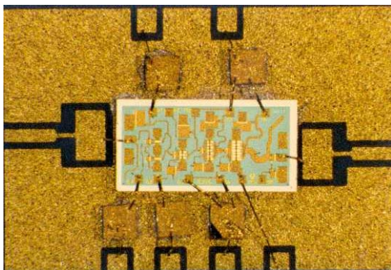
Fig. 1: Photo of the UMS GaAs medium power amplifier on DuPont 951 LTCC with co-fired Fodel™ gold conductor on top of the substrate
