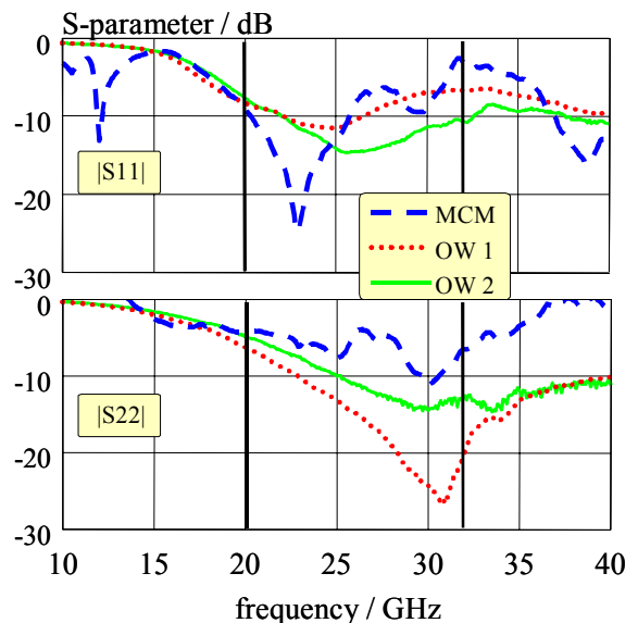
Fig. 8: Measured return losses of the LNA
